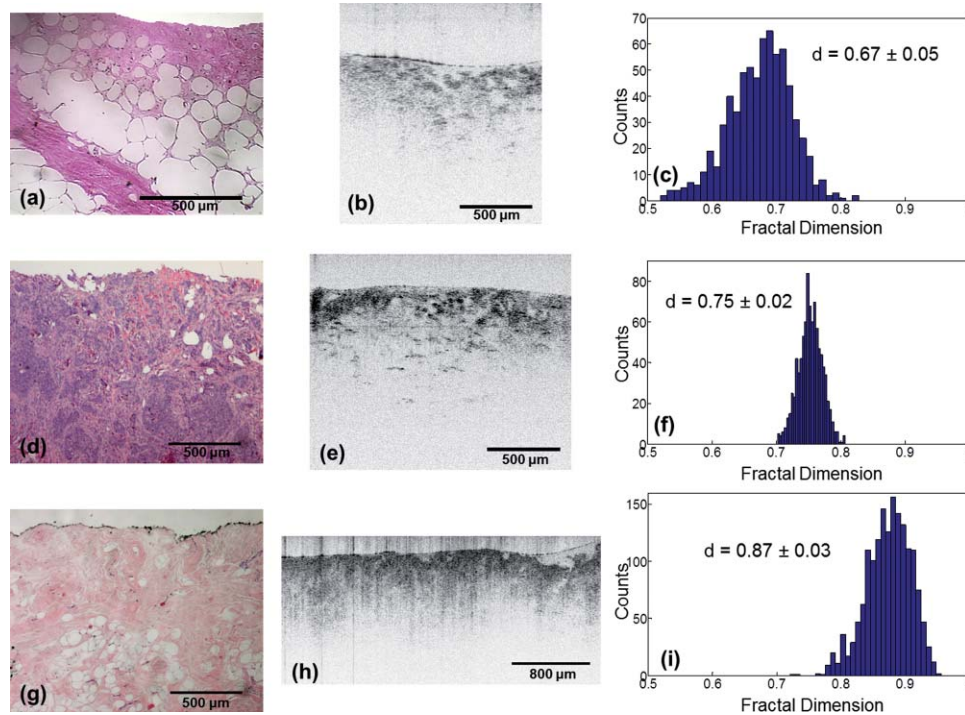
Fig. 2 Microscopy images of H&E stained breast tissue [(a), (d), and (e)], along with the corresponding B-mode OCT images [(b), (e), and (h)], and distributions of fractal dimension values [(c), (f), and (i)] for the entire region. The tissue classifications for these regions are adipose [(a)–(c)], cancer (invasive ductal carcinoma) [(d)–(f)], and stroma [(g)–(i)]. Stromal regions within the adipose tissue (a) and adipose cells within the cancer (d) and stromal tissues (g) are heterogeneities that may broaden the measured fractal dimension distribution.
