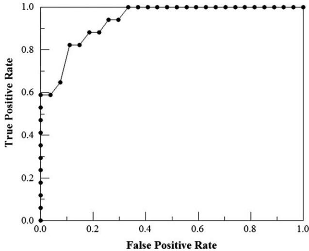
Fig. 3 ROC curve for a sensitivity and specificity test for classifying cancer versus adipose or stroma based on fractal dimension in OCT images. The area under the curve is calculated to be 0.938.
