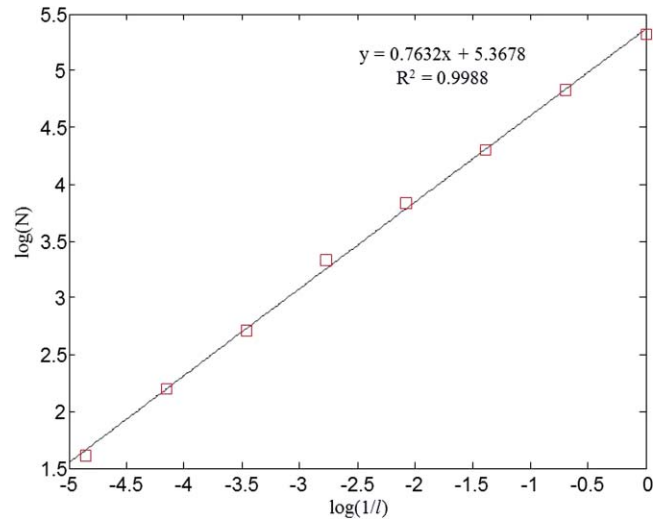
Fig. 1 A log-log plot of number of boxes versus box size for a single column. The slope of the linear fit is the fractal dimension.
